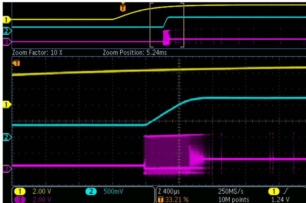
Pre-bias start up (~400mV), 12V Vin, 1.2V Vout (Ch2), SW (Ch3), Vin(Ch1)
