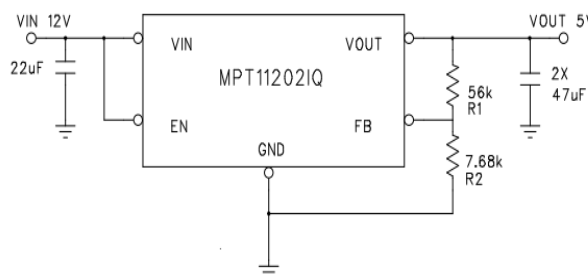
Figure 1: Simplified Applications Circuit
