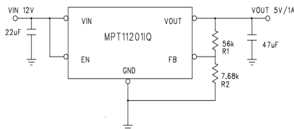
Figure 1: Simplified Applications Circuit
