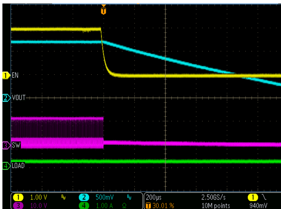
Shutdown, 12V Vin, 1.2V Vout, No LOAD
