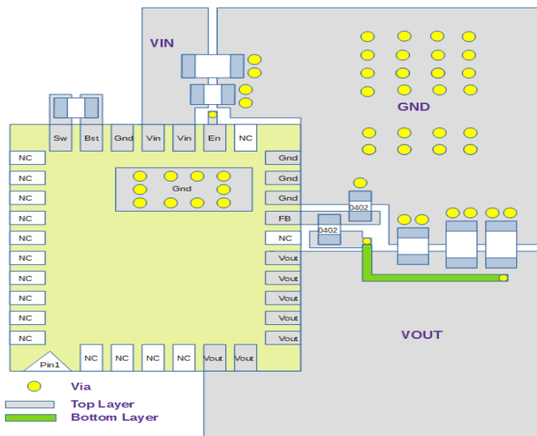
Figure 6: Recommended PCB Layout
