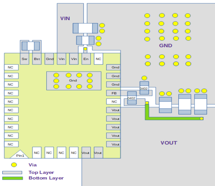
Figure 6: Recommended PCB Layout
