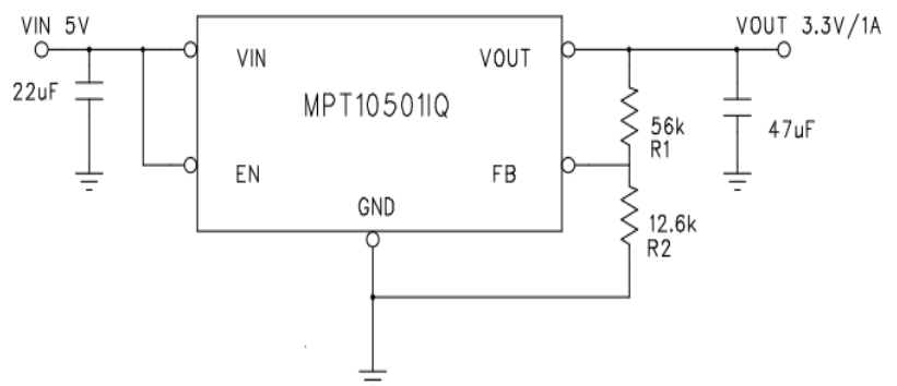
Figure 4: Simplified Applications Circuit
