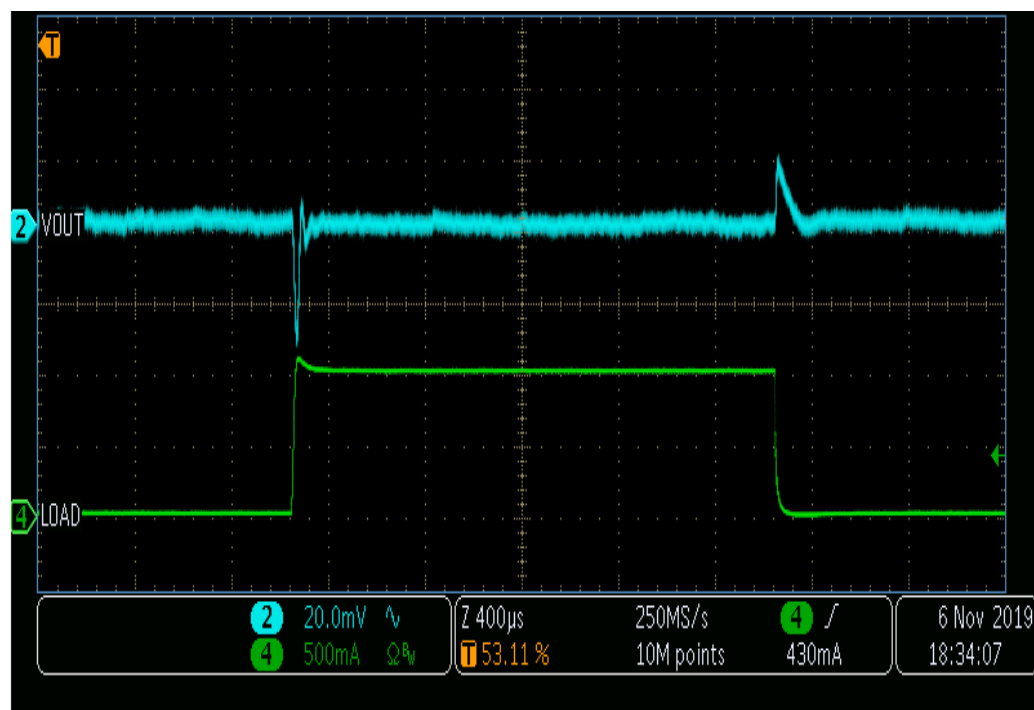
Load Transient Response, 5V Vin, 1.2V Vout, 1A DC LOAD
