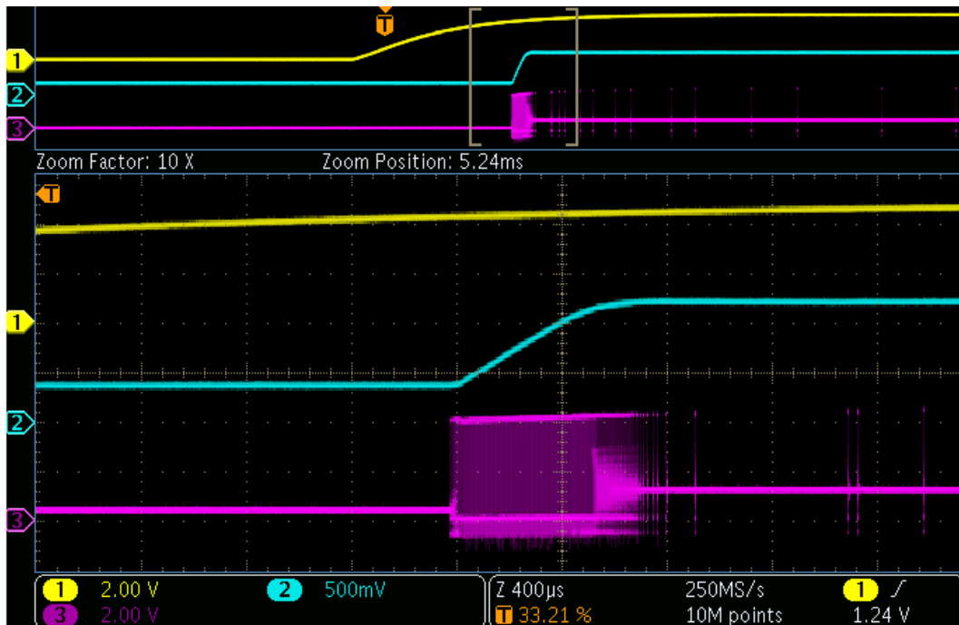
Pre-bias start up (~400mV), 5V Vin, 1.2V Vout Vout (Ch2), SW (Ch3), Vin(Ch1)
