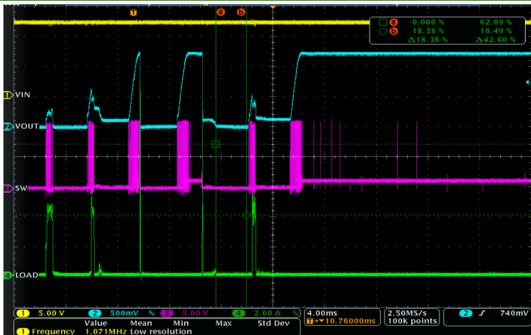
Short Circuit RECOVERY, 5V Vin, 1.2V Vout
