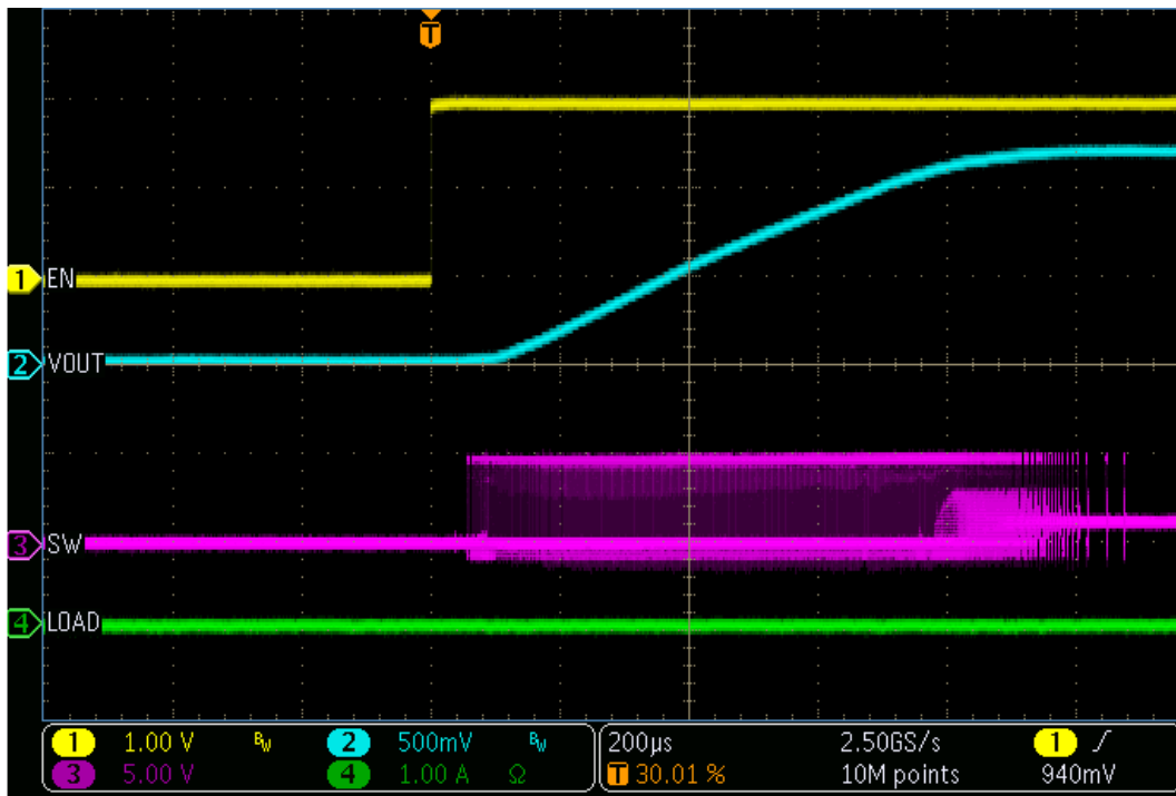
Startup, 5V Vin, 1.2V Vout, No LOAD
