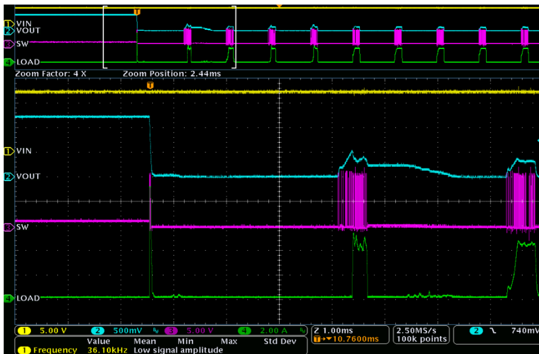
Short Circuit RESPONSE, 5V Vin, 1.2V Vout
