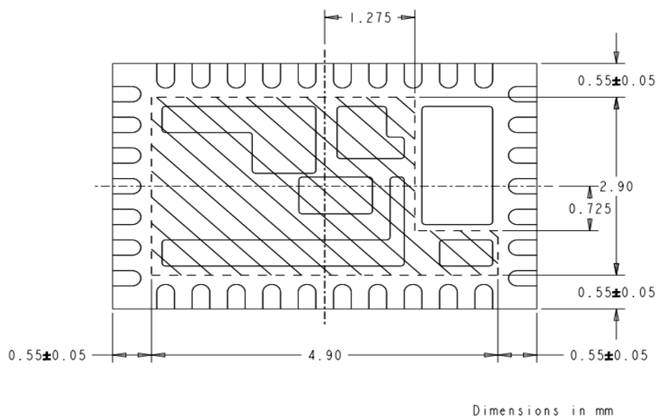
Figure 7: Lead-Frame exposed metal (Bottom View)
