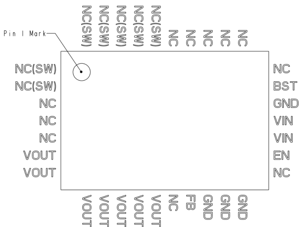
Figure 1: Pin Diagram (Top View)
