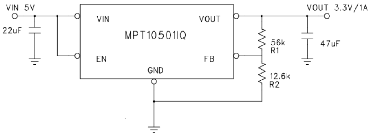
Figure 5: Typical Application Circuit
