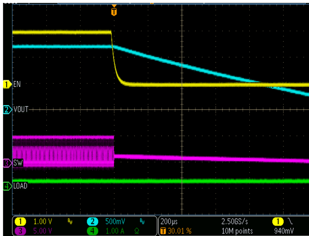
Shutdown, 5V Vin, 1.2V Vout, No LOAD
