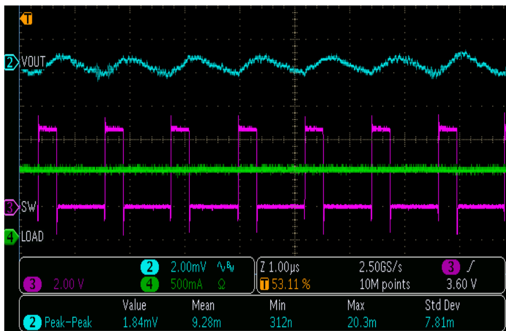
OUTPUT Ripple, 5V Vin, 1.2V Vout, 1A DC LOAD
