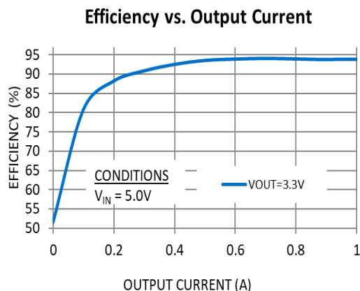
Figure 3: Efficiency at 5V Vin; 3.3V Vout
